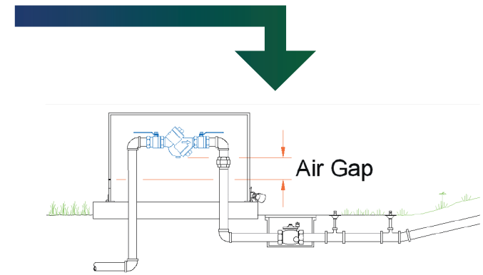
Reduced Pressure Backflow Assembly in Above-Ground Enclosure
