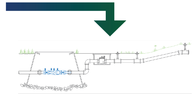
Double Check Valve Assembly in Below-Ground Box
