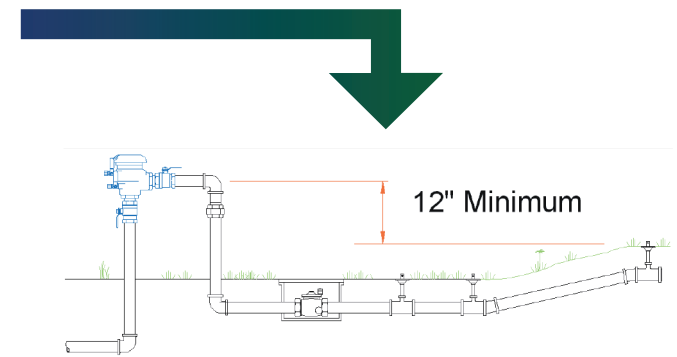
Pressure Vacuum Breaker Assembly
