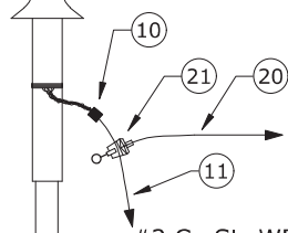
Pothead Connection Detail
